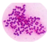
Rothia aeria
