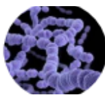
Streptococcus australis
